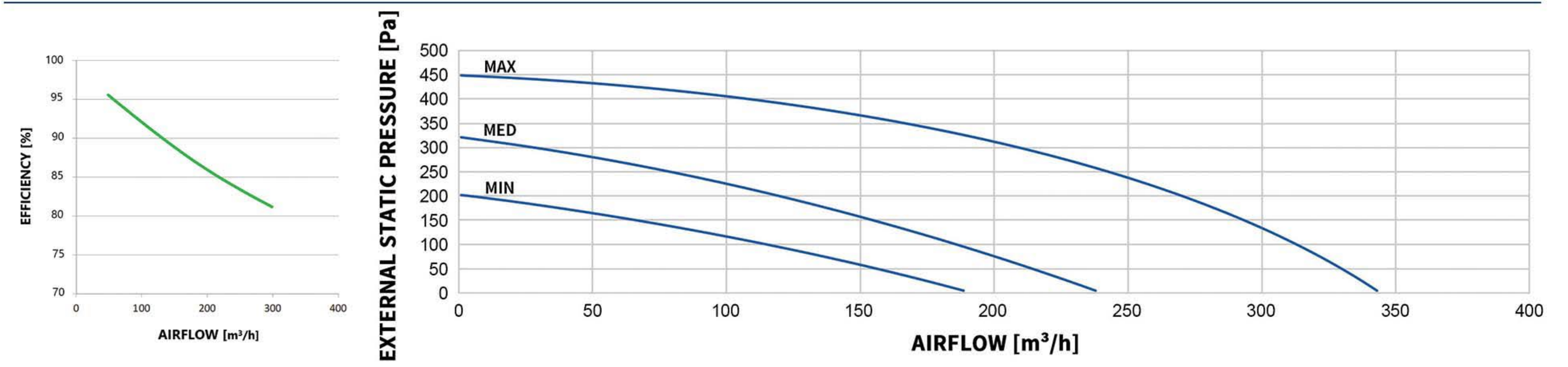
MODEL: W300-ERV-B-Z-EC
