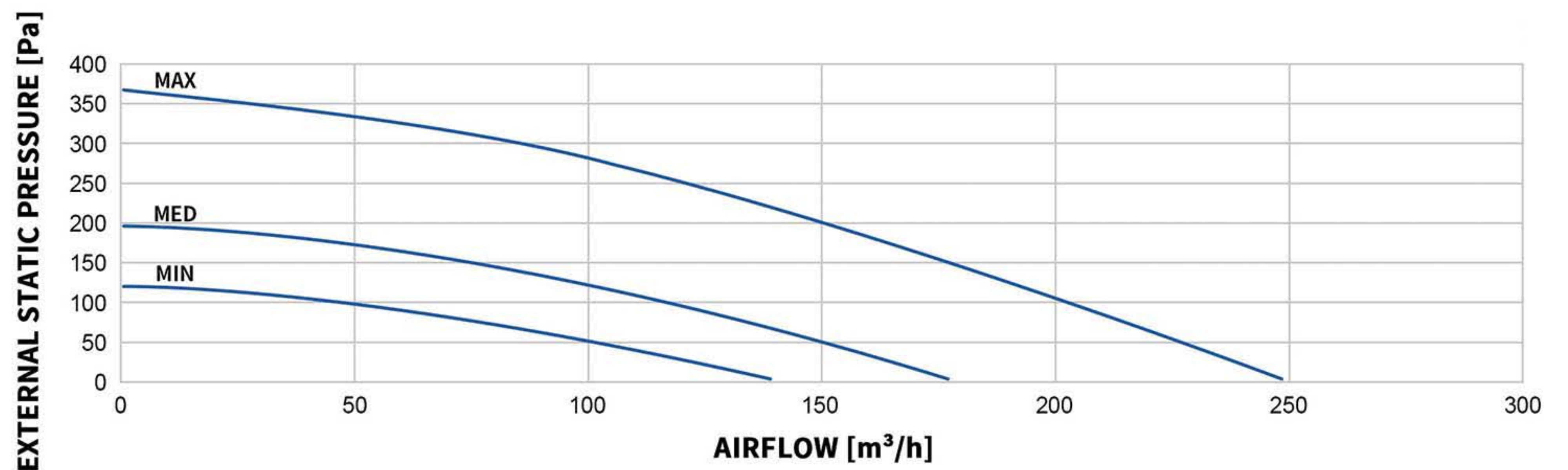
MODEL: W240-ERV-B-Z-EC
