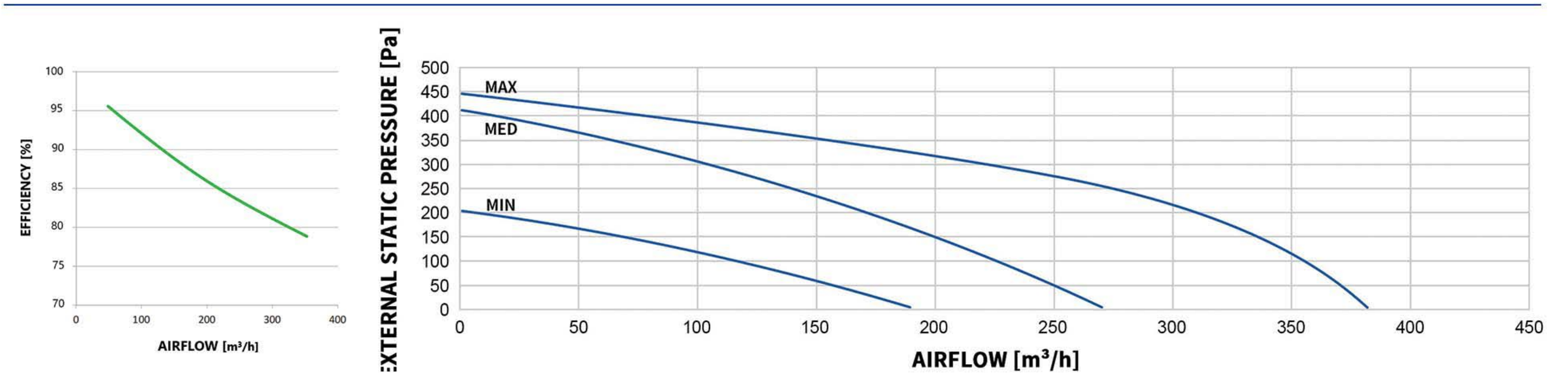
MODEL: W350-ERV-B-Z-EC
