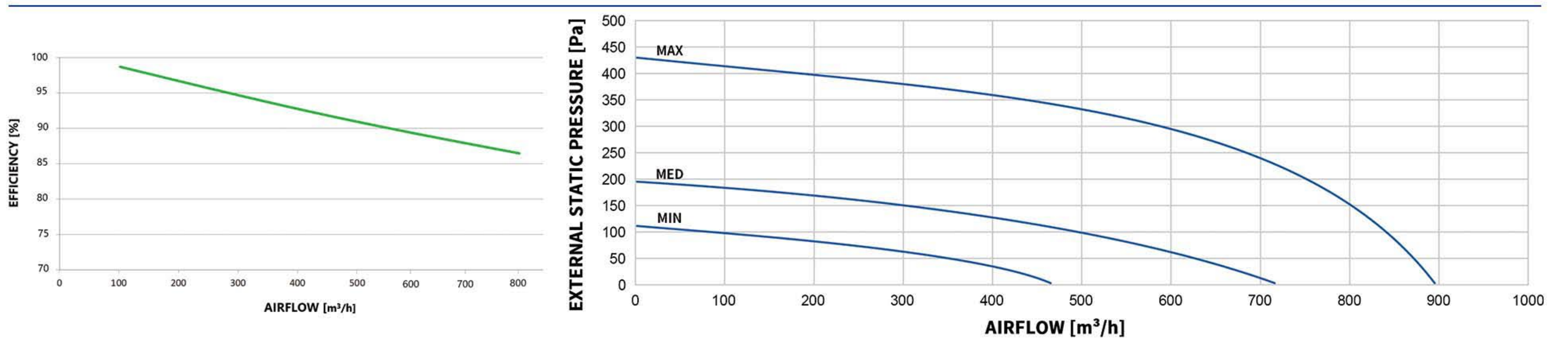
MODEL: W800-ERV-B-Z-EC
