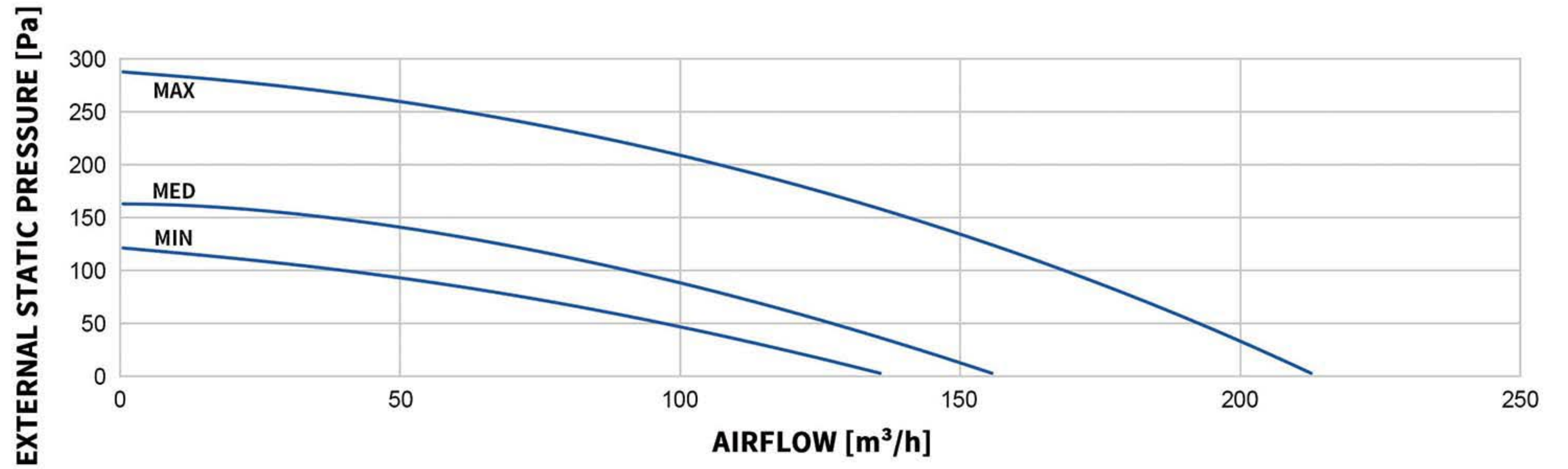
MODEL: W190-ERV-B-Z-EC
