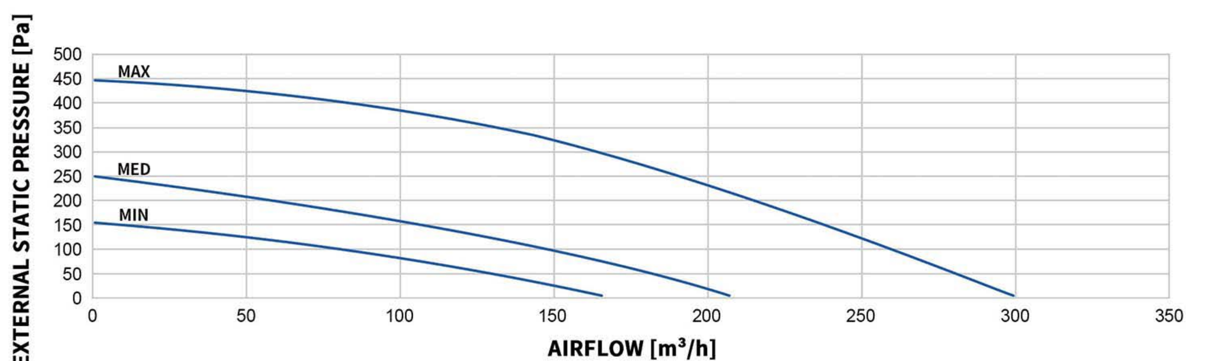
MODEL: W250-ERV-B-Z-EC
