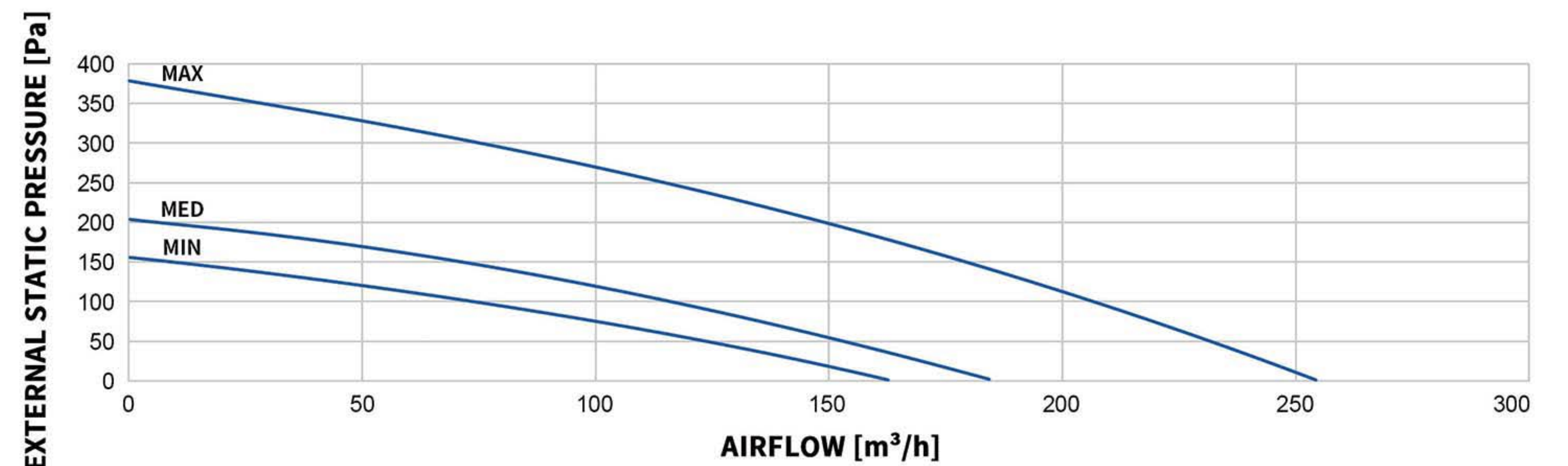
MODEL: W200-ERV-B-Z-EC
